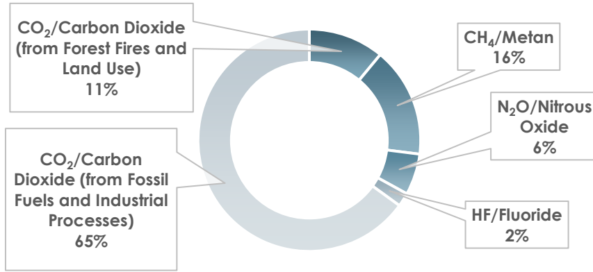
Figure 1. Effects of Different Greenhouse Gases on Global Warming
